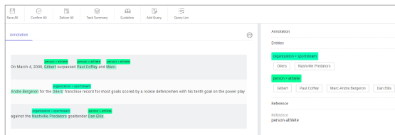
Figure 4: Screenshot of the interface used to annotate FIEE-NERD.
